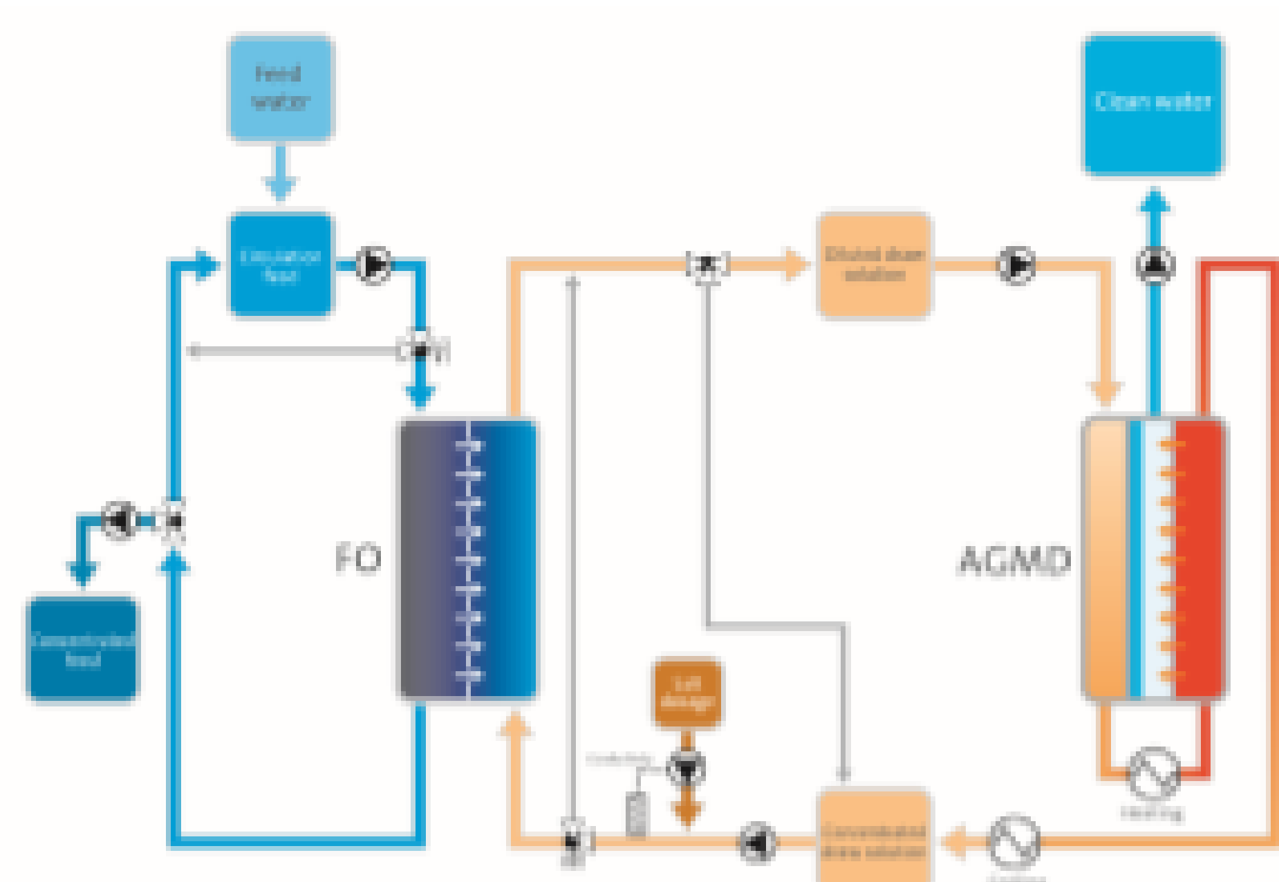
Forward Osmosis with Membrane Distillation flow scheme
