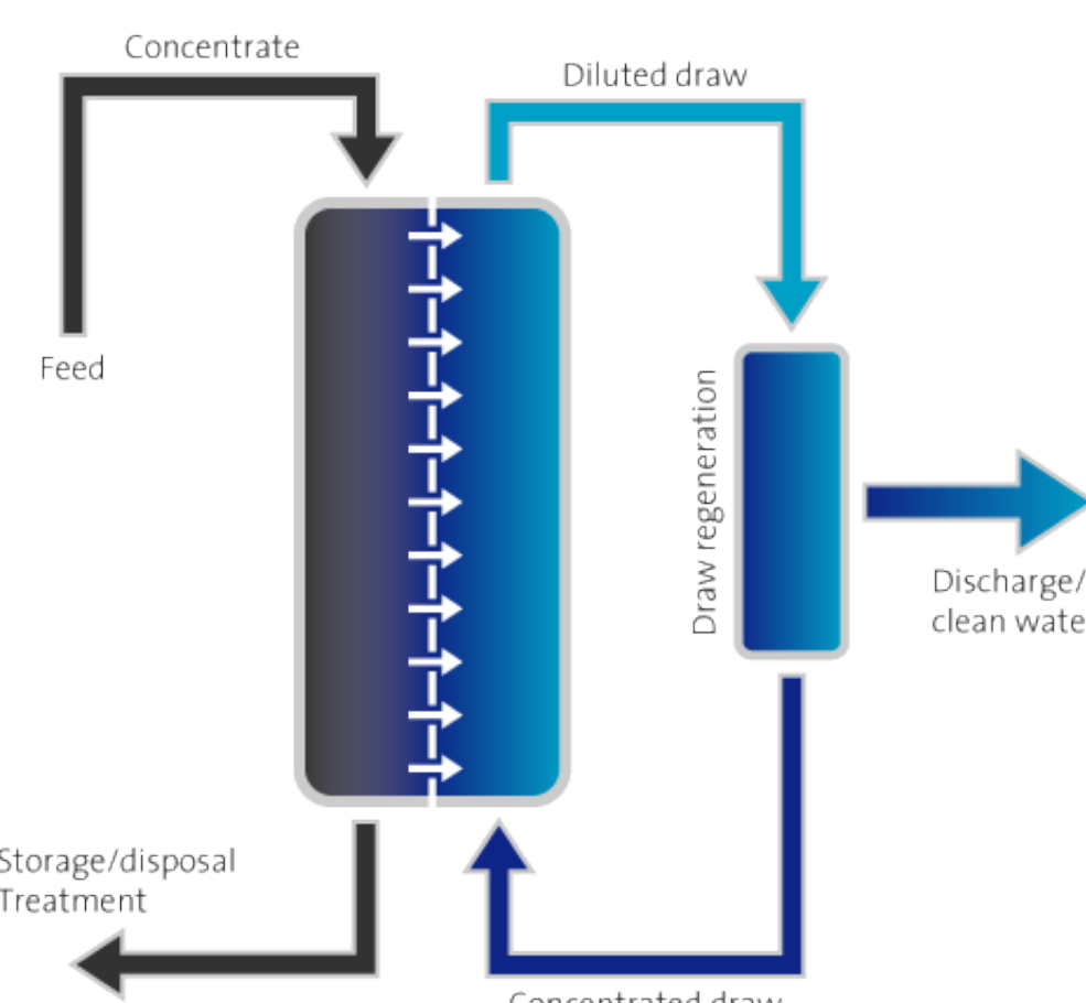
FO with draw solution recovery
